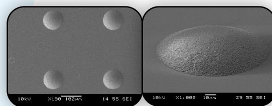
100 μm diameter adhesive dot
