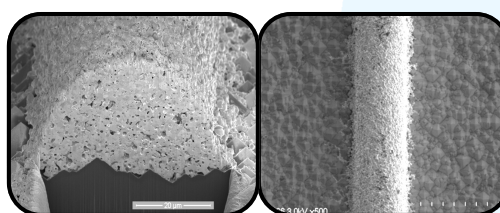
50 μm wide conductive lines with high aspect ratio
